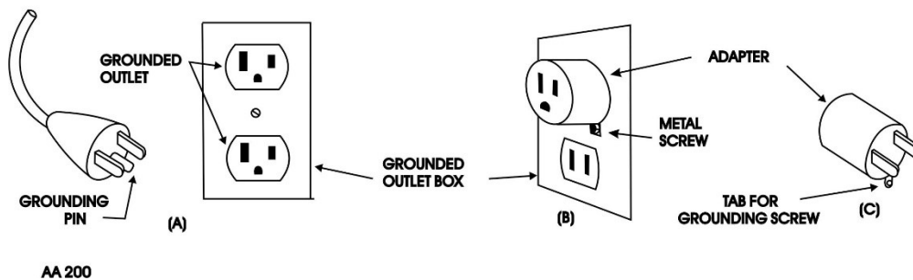
Figure 1. Grounding methods
