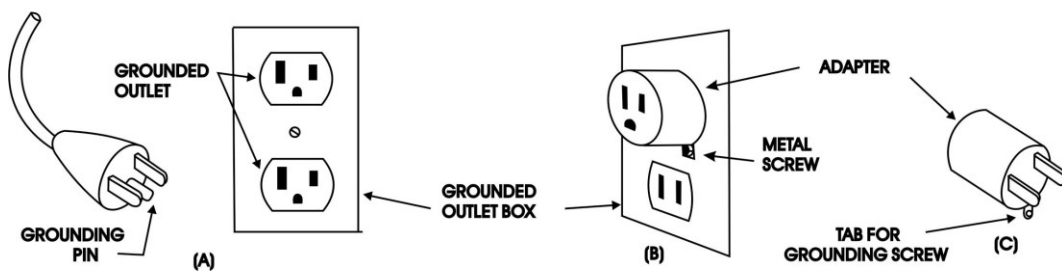
Grounding methods
